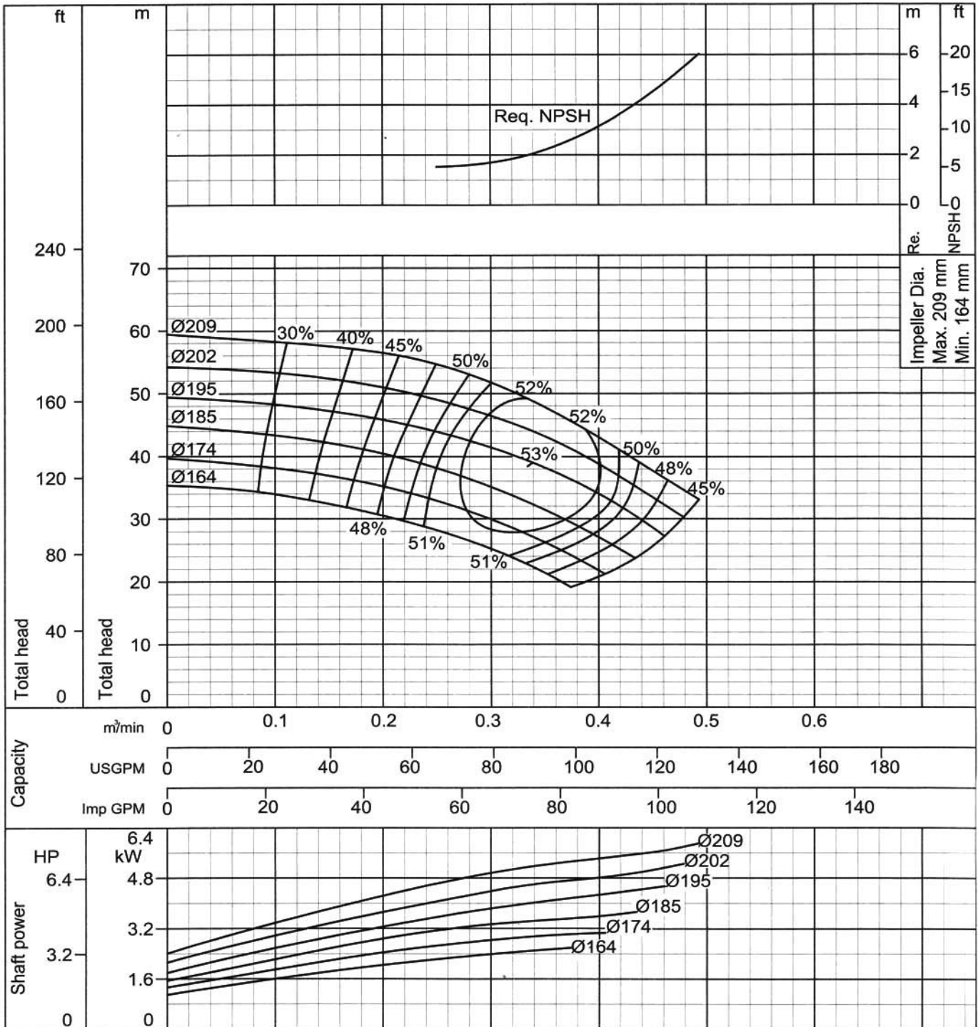
Curve No - 2 - 5FS5601R1
