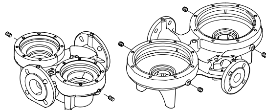
Fig. 24 Tappings for mounting of automatic air vents in TP Series 200 and TP Series 300
