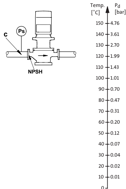
Fig. 40 Minimum inlet pressure
