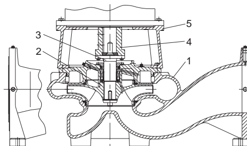
Fig. 8 Sectional drawing of TP Series 400
