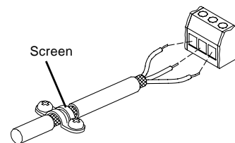
Fig. 33 External start/stop cable connection of TPE, TPED
