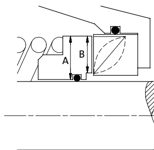
Fig. 7 Areas where the forces of an unbalanced seal act
