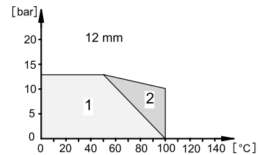
Fig. 37 Pressure/temperature diagrams
