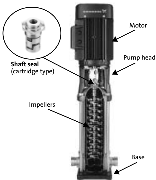
Fig. 1 Shaft seal in a CR pump (in-line pump)
