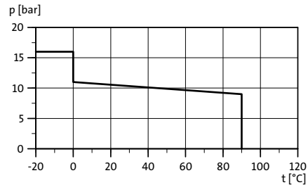
Fig. 44 Pressure/temperature diagram
