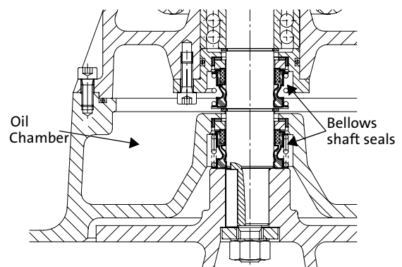
Fig. 58 Tandem seal arrangement in an AP pump
