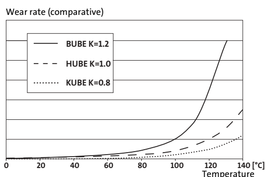
Fig. 12 Wear rate for different balancing ratios
