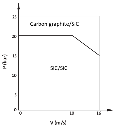
Fig. 63 Pressure/velocity of seal face diagram
