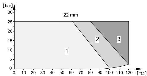
Fig. 42 Pressure/temperature diagrams
