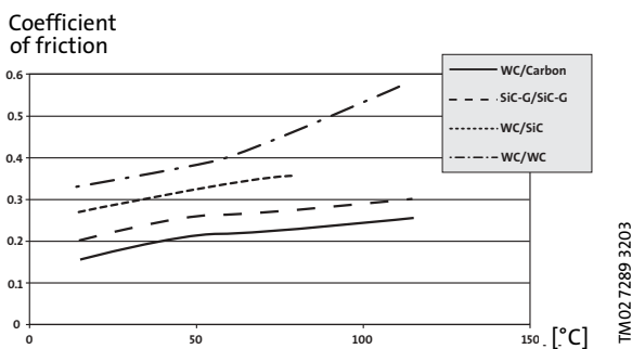
Fig. 29 Start friction in water
