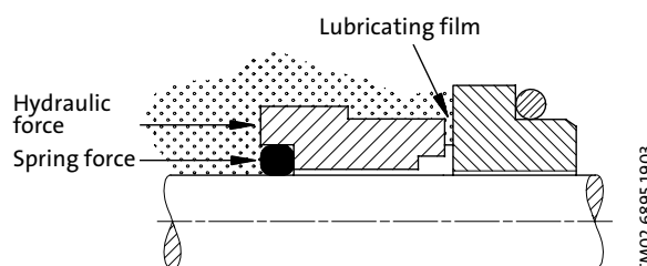
Fig. 3 Rotating shaft seal
