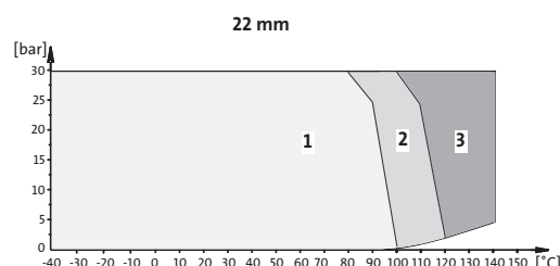
Fig. 46 Pressure/temperature diagrams
