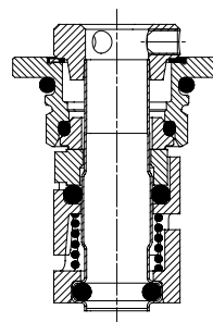
Fig. 18 Cartridge shaft seal
