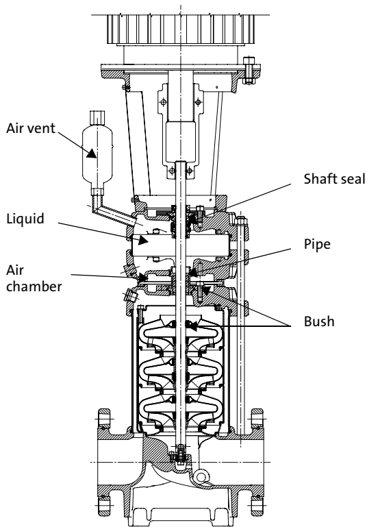
Fig. 65 Drawing of a CR pump with an air-cooled top assembly
