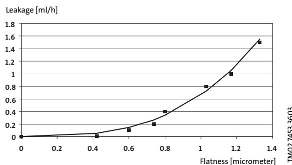
Fig. 13 Flatness as a function of leakage
