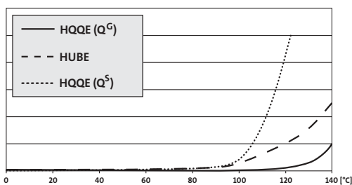
Fig. 24 Wear rate of seal faces
