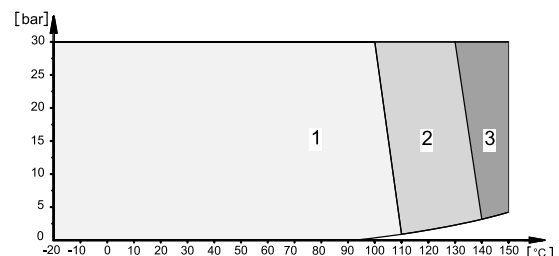
Fig. 51 Pressure/temperature diagrams
