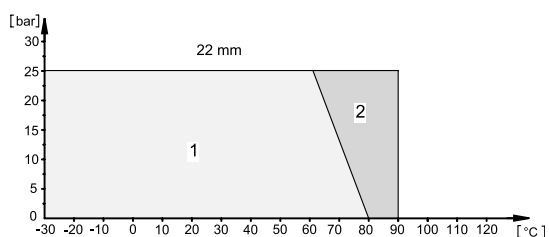
Fig. 41 Pressure/temperature diagrams
