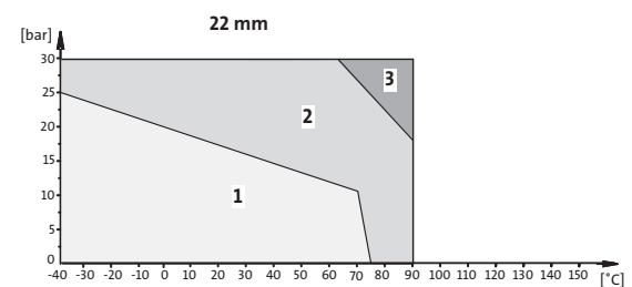
Fig. 49 Pressure/temperature diagrams
