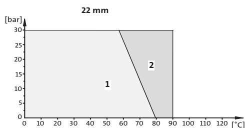
Fig. 53 Pressure/temperature diagrams
