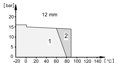
Fig. 55 Pressure/temperature diagrams
