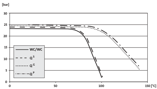
Fig. 23 Limits for stable friction of a seal
