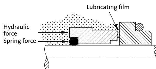
Fig. 10 Shaft seal during operation
