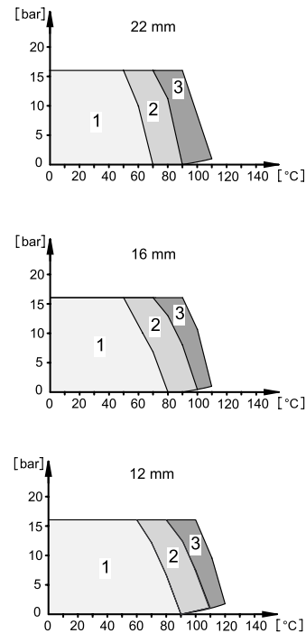
Fig. 35 Pressure/temperature diagrams
