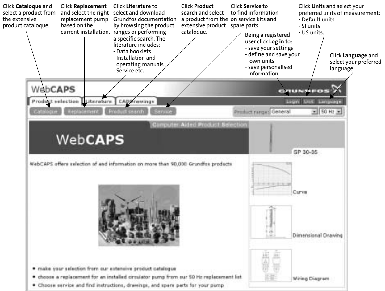
Fig. 68 WebCAPS
