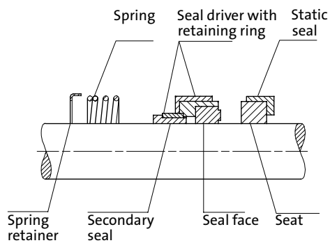
Fig. 4 Components of mechanical shaft seals
