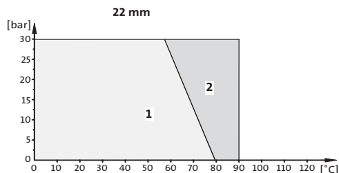
Fig. 52 Pressure/temperature diagrams
