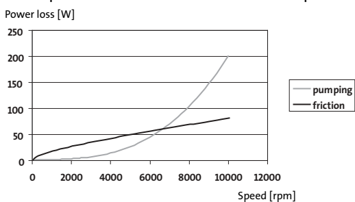
Fig. 11 Power consumption of seal
