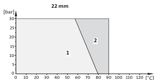
Fig. 40 Pressure/temperature diagrams
