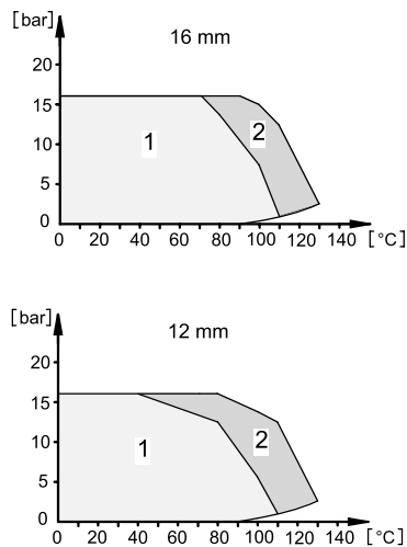
Fig. 34 Pressure/temperature diagrams
