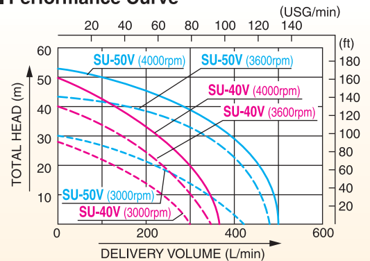
■ Performance Curve
