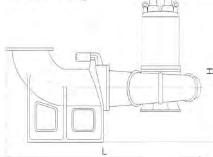
Guide Rail Fitting
