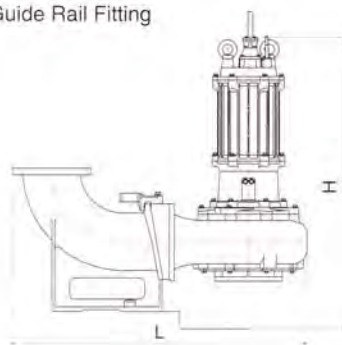
Guide Rail Fitting
